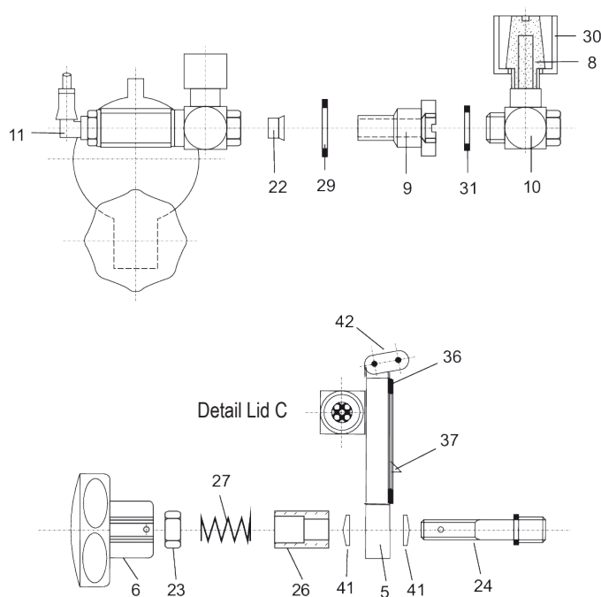
Detail Locking
