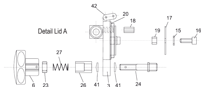
Detail Locking
